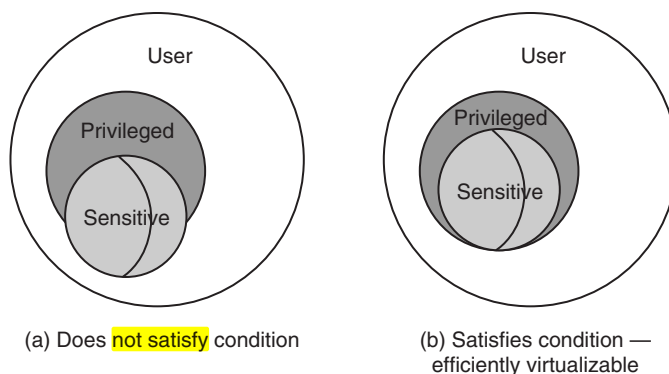
Figure 8.8 Illustrating Popek and Goldberg's Theorem 1 . In (a), the sensitive instructions are not a subset of the privileged instructions and hence the system may not be efficiently virtualizable. On the other hand, the system in (b) satisfies the condition of Theorem 1.
